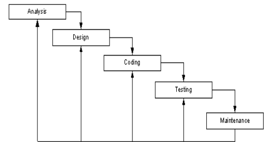
Gambar 2. Tahapan waterfall
