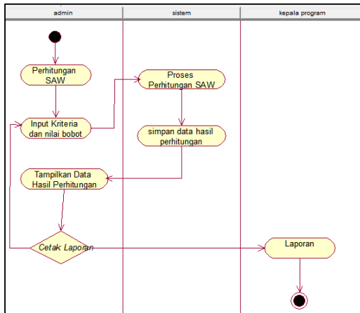
Gambar 3 Activity Diagram Perhitungan SAW
