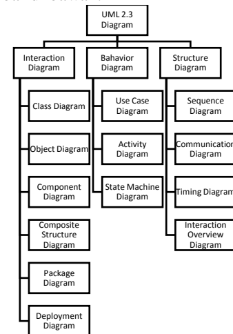
Gambar 1. Diagram UML
